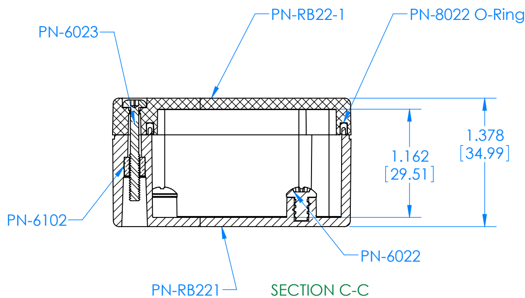
SECTION C-C
