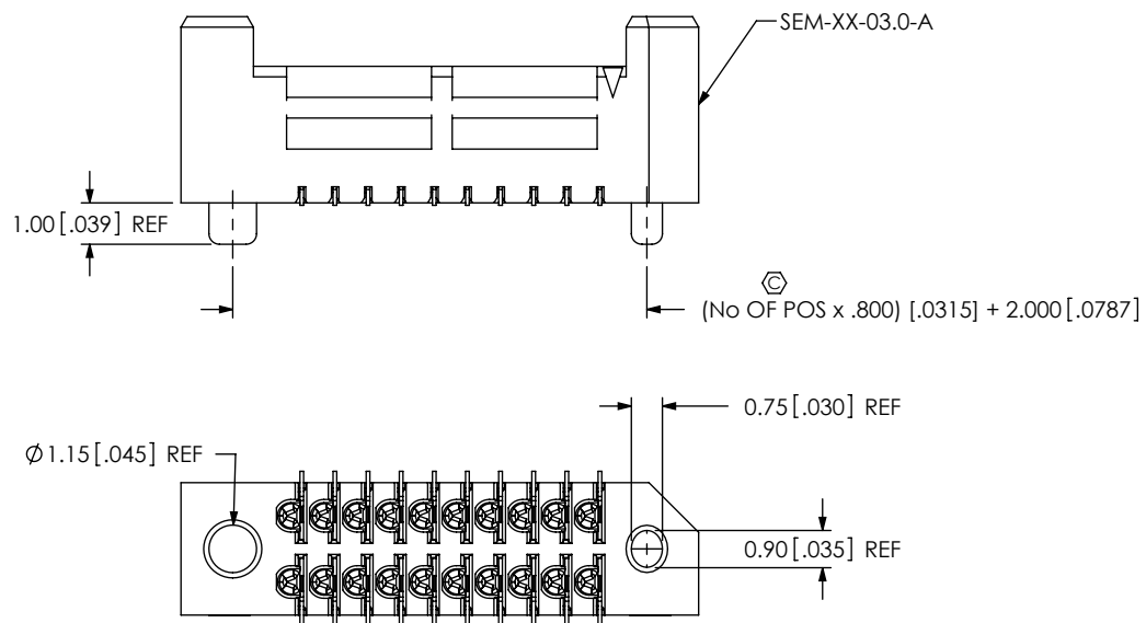
FIG 2 SEM-110-02-03.0-XX-D-A SHOWN
