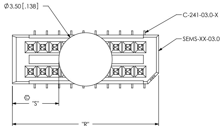
FIG 7 SEMS-110-02-03.0-XX-D-K SHOWN
