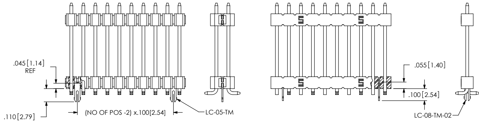
FIG 2 -LC: LOCKING CLIP (SAME AS FIG 1, DIFFERENT AS SHOWN)
