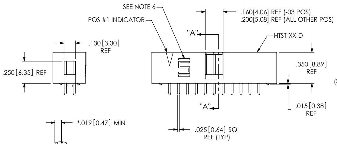
FIG 1 HTST-111-0T-XX-D-LL SHOWN * DIMENSIONS APPLY WHEN USING -LL OPTION ONLY
