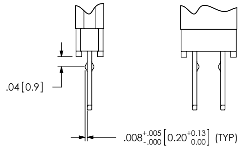
FIG 4 LOCKING LEAD OPTION LOCATED ON OR ABOUT THE CENTERLINE (N/A IN 1 OR 2 POSITION SINGLE ROW)
