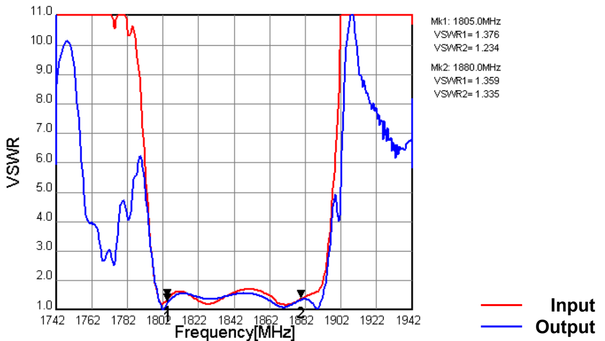
Fig.10 VSWR (Filter2)
