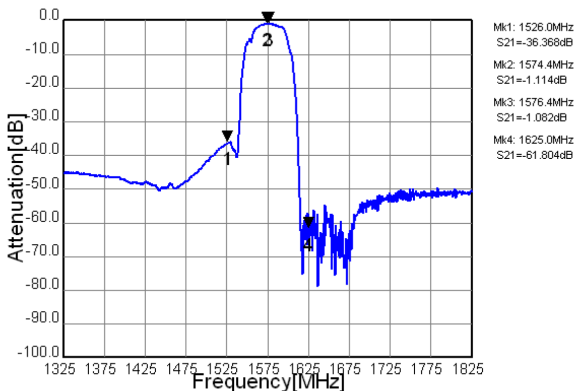
Fig.1 Pass-band Characteristics
