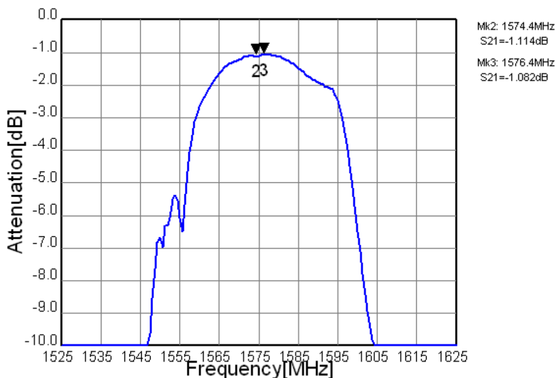
Fig.3 In-band Characteristics
