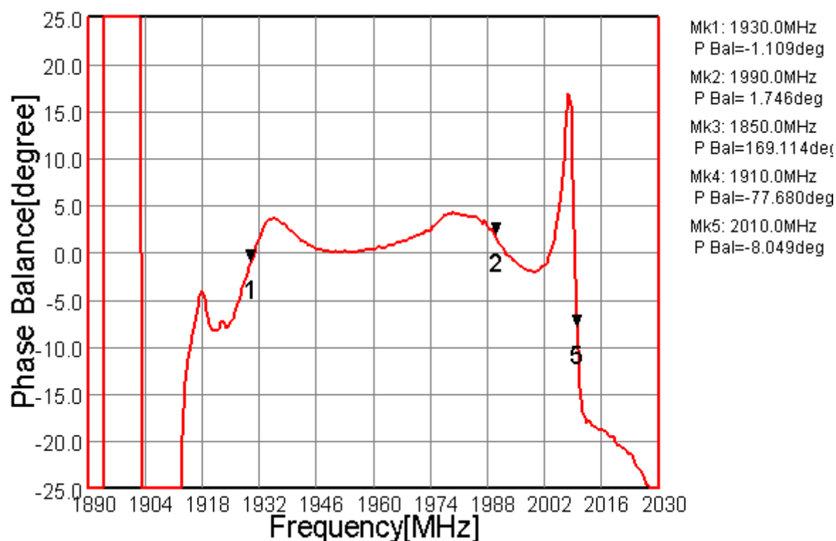
Fig.8 Phase Balance
