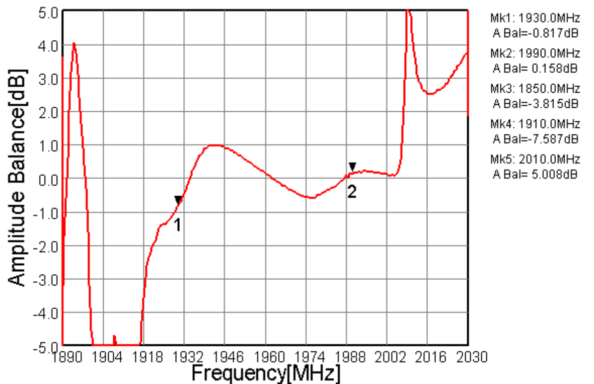
Fig.7 Amplitude Balance
