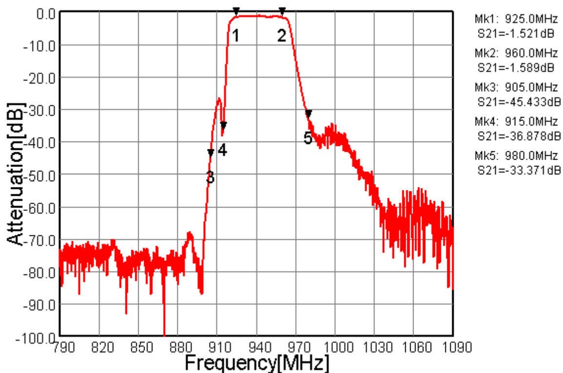
Fig.1 Pass-band Characteristics
