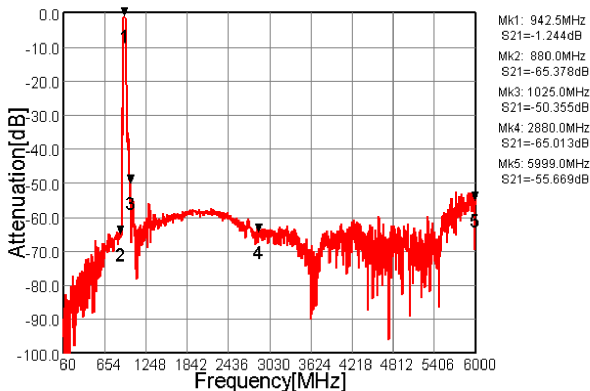
Fig.4 Wide-band Characteristics
