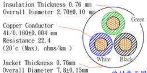
線材截面圖 (Wire Cross-Section)
