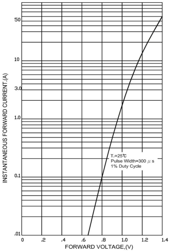
FIG.3-TYPICAL FORWARD CHARACTERISTICS
