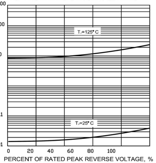
FIG.4-TYPICAL REVERSE CHARACTERISTICS PER LEG
