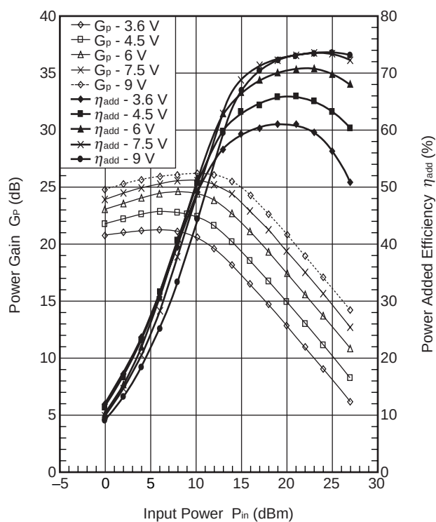
POWER GAIN, POWER ADDED EFFICIENCY vs. INPUT POWER
