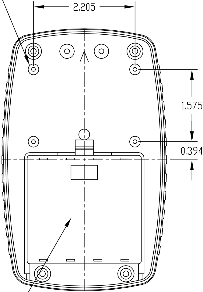
INSIDE VIEW OF BOTTOM
