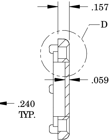
SECTION C-C
