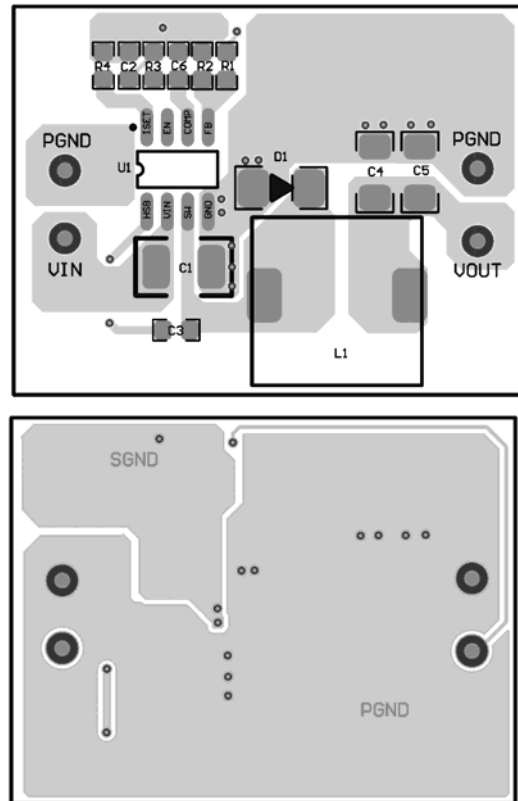
Figure 8: PCB Layout
