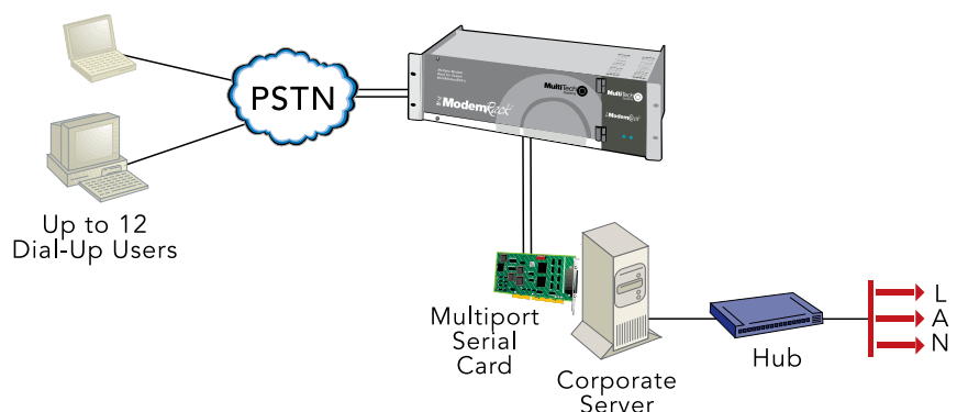
Multiport serial cards connect to modems in ZDXRack for dial-up users.
