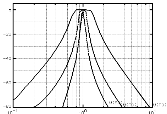
Bandpass Responses
