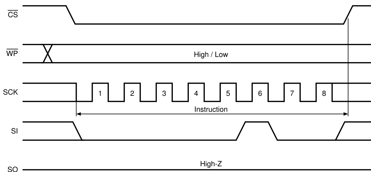
Figure 12 WRDI Operation
