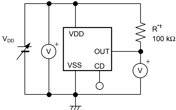
Figure 6 Test Circuit 1
