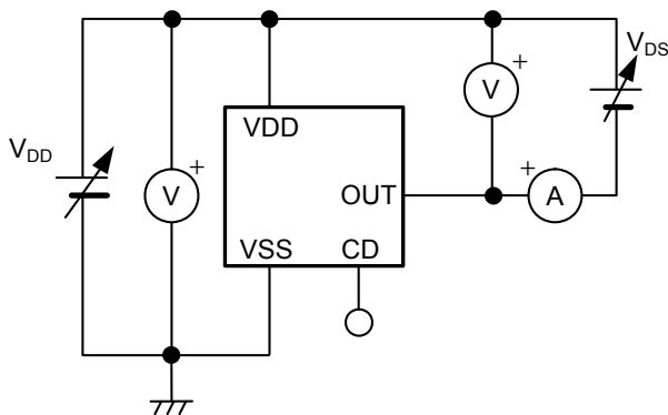
Figure 10 Test Circuit 5
