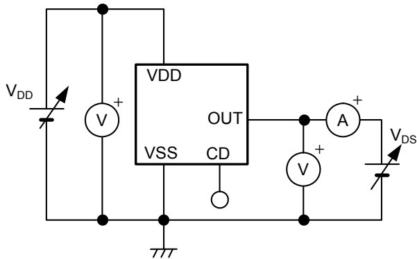
Figure 8 Test Circuit 3
