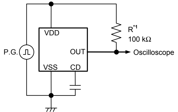
Figure 9 Test Circuit 4
