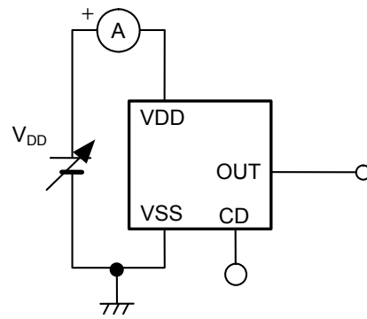
Figure 7 Test Circuit 2
