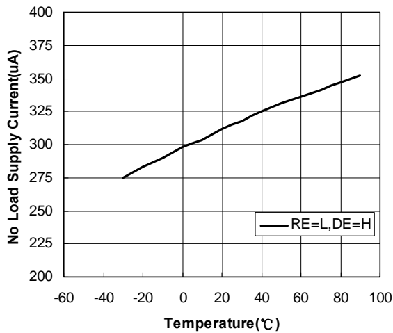
No Load Supply Current vs. Temperature
