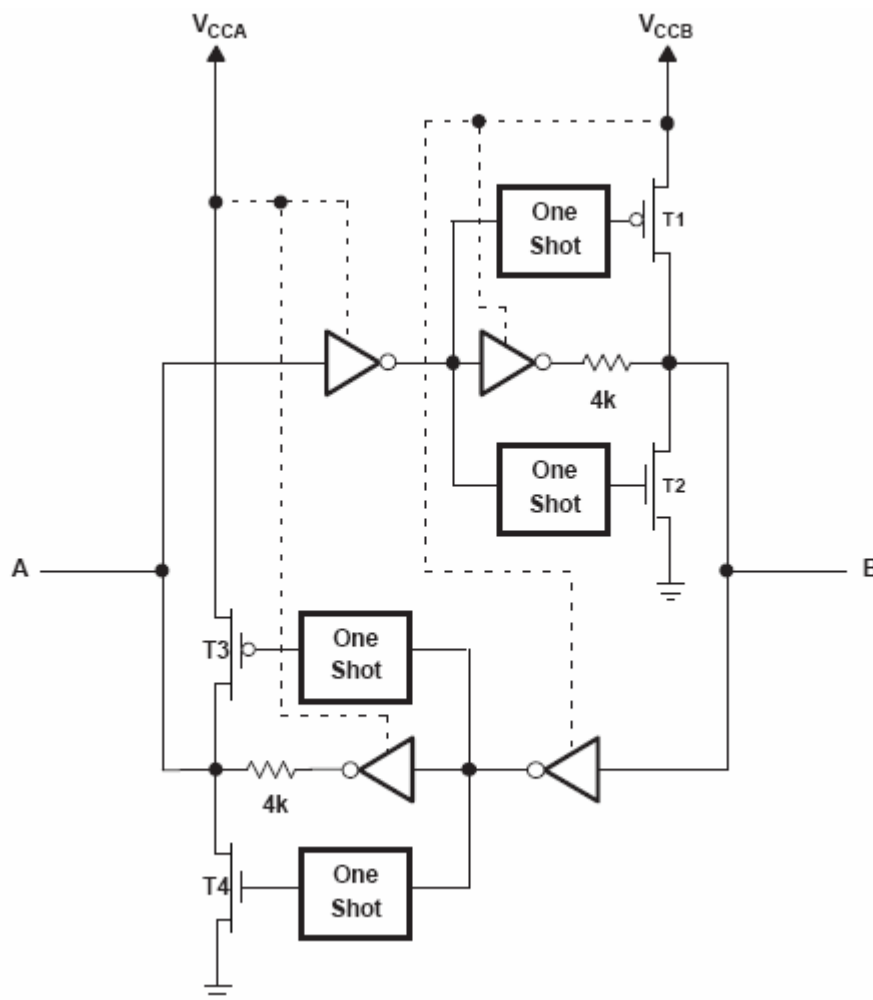
Figure 1 Block Diagram of UM3304/UM3304Q/UM3304QT I/O Cell
