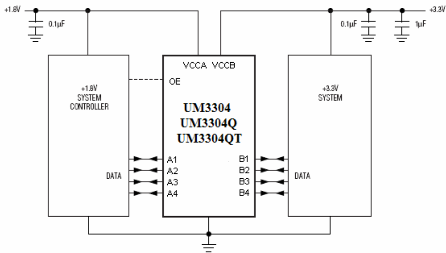
Figure 3 Typical operating circuit
