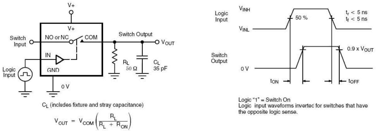
FIGURE 1. Switching Time
