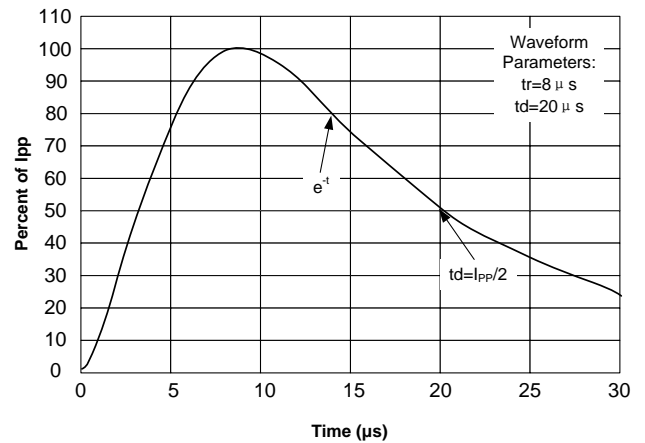
Pulse Waveform
