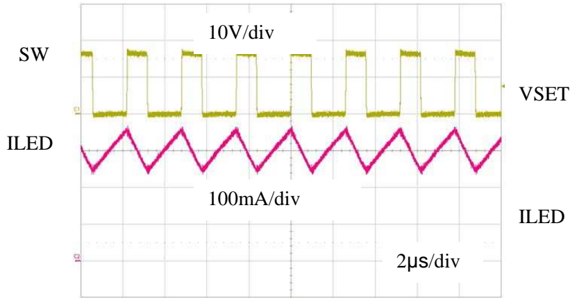
Steady State Waveforms (3LEDs, 100uH, Vin=16V, Rs=0.33Ω)
