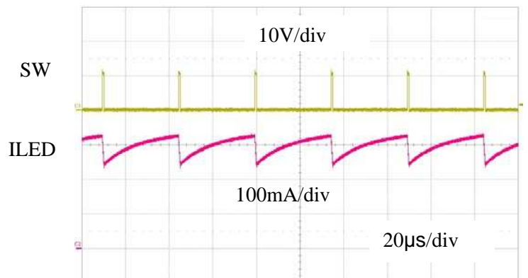
Pulse Skip Mode (3LEDs, 100uH, Vin=10V, Rs=0.33Ω)
