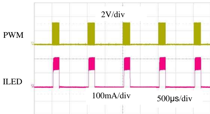
Dimming Waveforms (PWM=50%, 3LEDs, 100uH, Vin=16V, Rs=0.33Ω)
