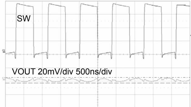
Heavy Load Operation ( V_{out}=1.8V , I_o=200mA )
