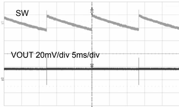
Light Load Operation ( V_{out}=1.8V , I_o=0mA )
