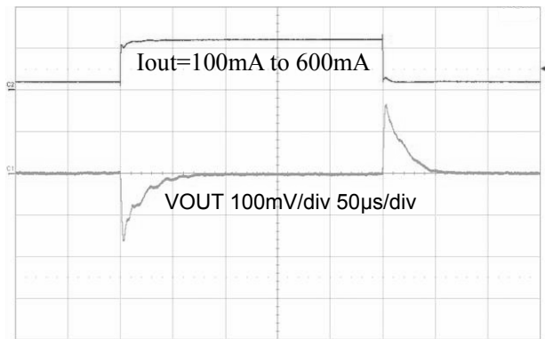
Load Transient Response ( V_{in} = 3.6V , V_{out} = 1.8V )
