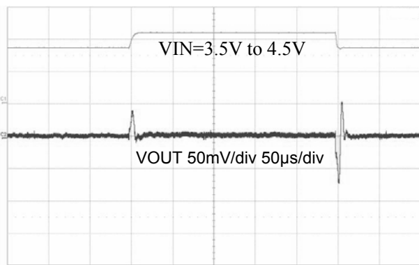
Line Transient Response ( V_{out} = 1.8V , I_{out} = 300mA )
