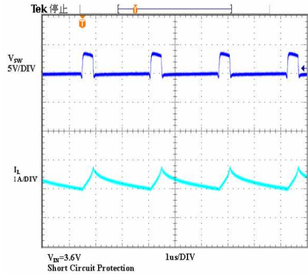
Short-Circuit Protection
