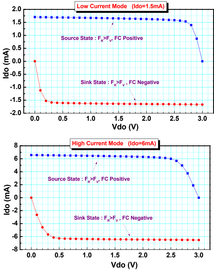
Fig. 7 – Charge pump current vs. V_{DO}
