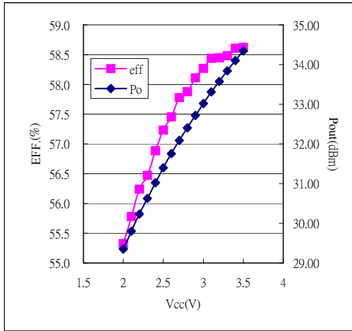
Fig 4.1 Output Power vs. Vcc
