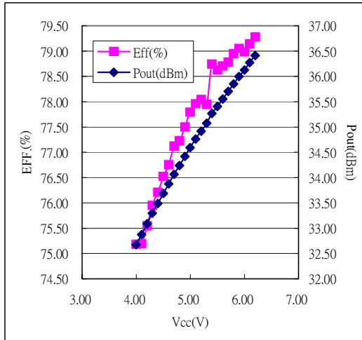
Fig 1.1 Output Power vs. Vcc
