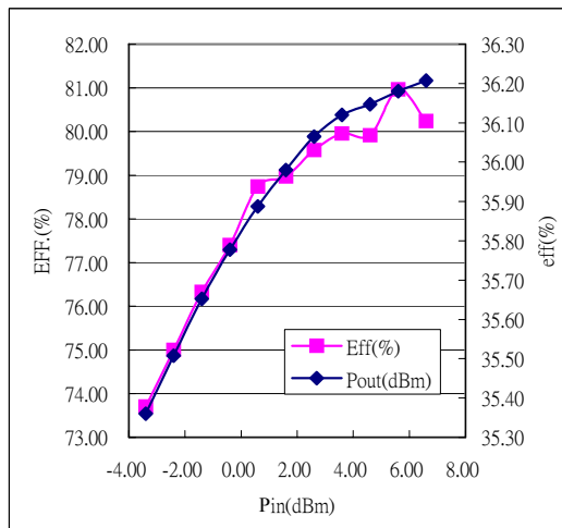
Fig 1.3 Output Power vs. Input Power
