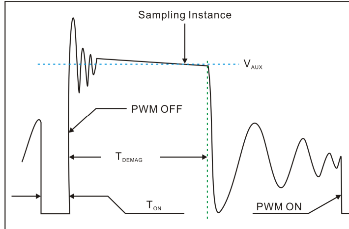
Figure 2. Auxiliary voltage waveform
