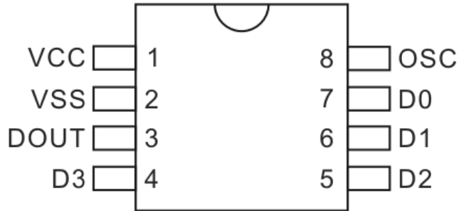
PT2240B
