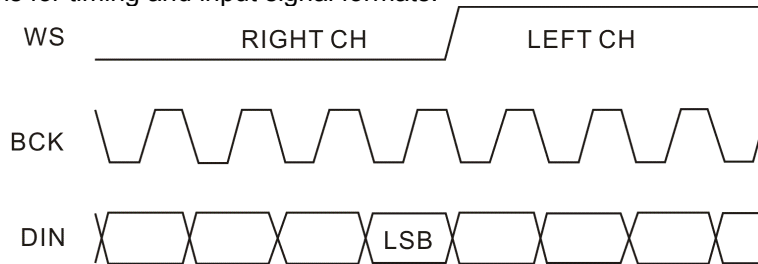
Figure 1. Japanese Input Signal Format
