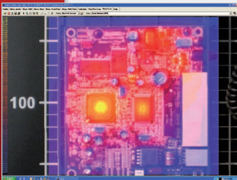
Heat measurement
