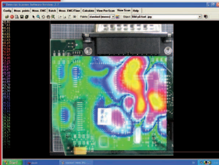
Scan measurement
