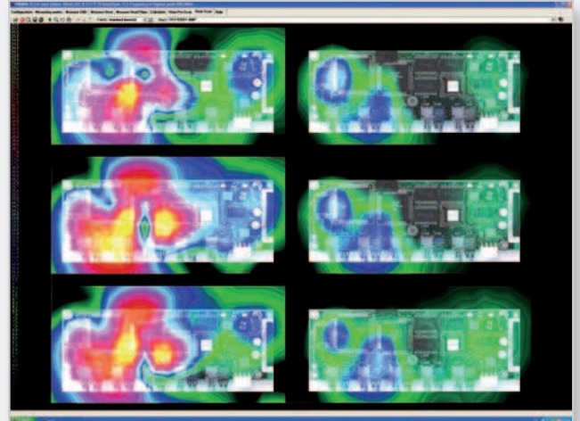
Six Scan measurements with different de-coupling
