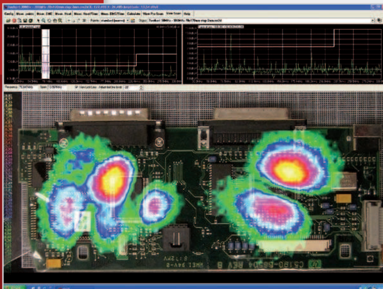
MultiScan measurement
