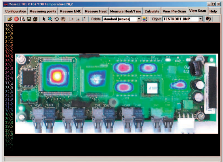
Heat measurement
