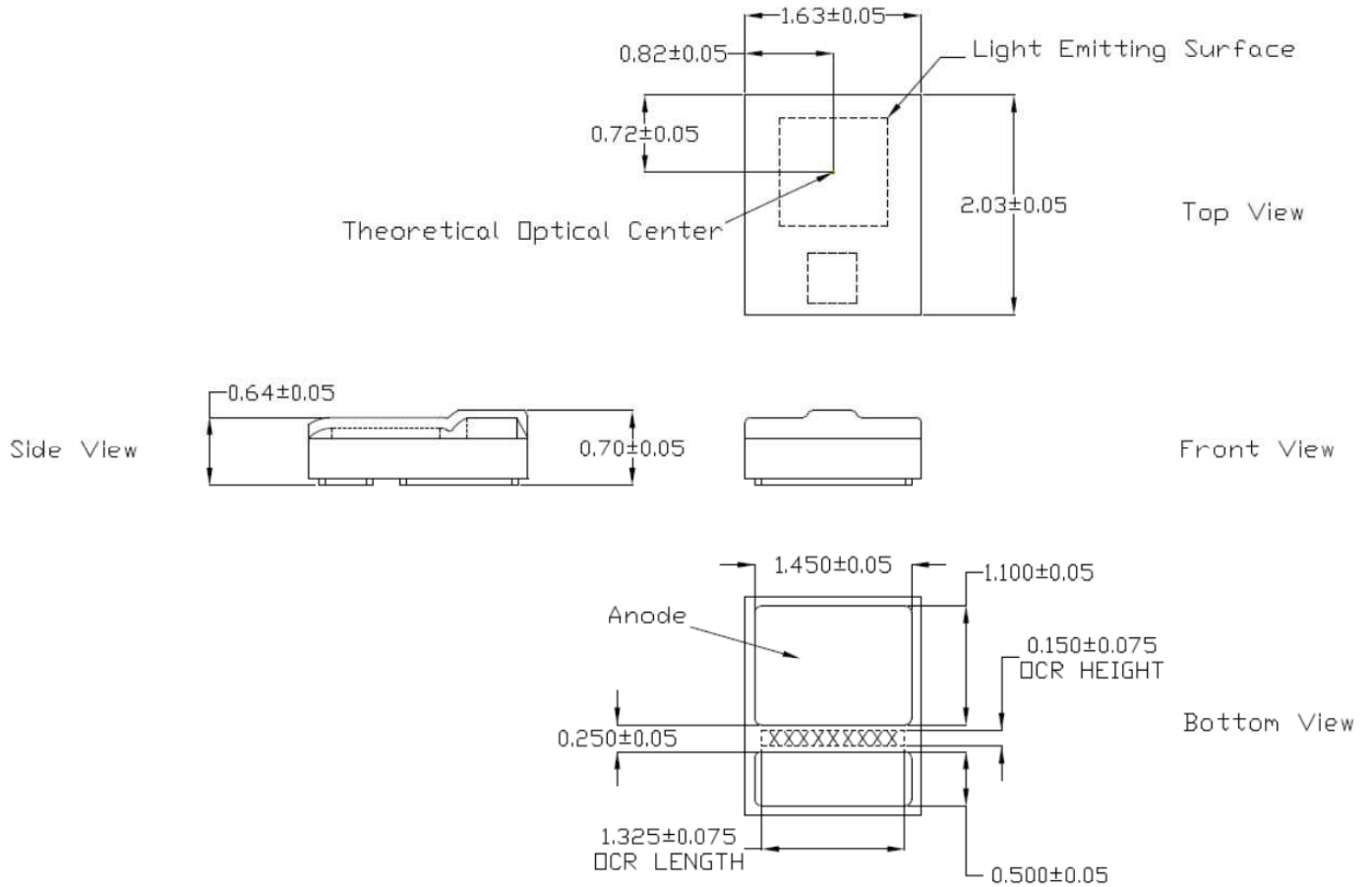
Figure 3. Dimensions for LXCL-EY17-xxxx.
