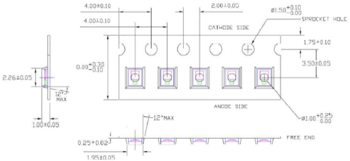
Figure 16. Tape dimensions.
