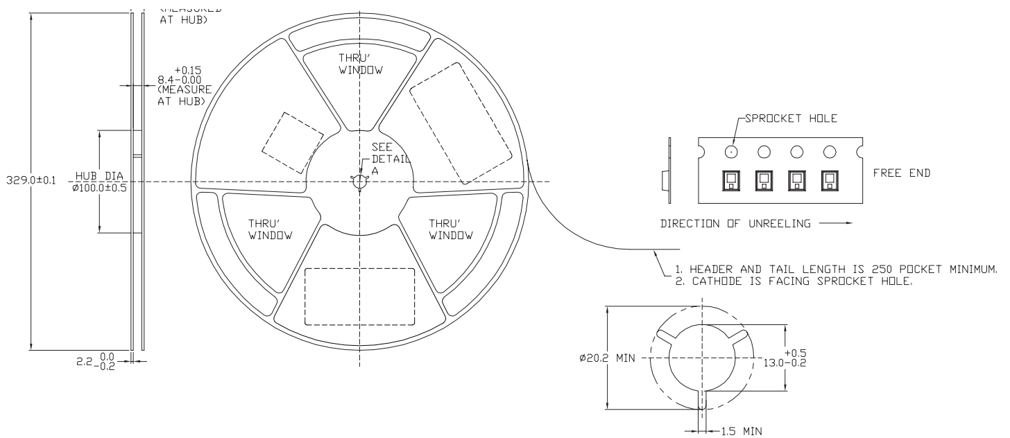
Figure 17. Emitter reel packaging.
