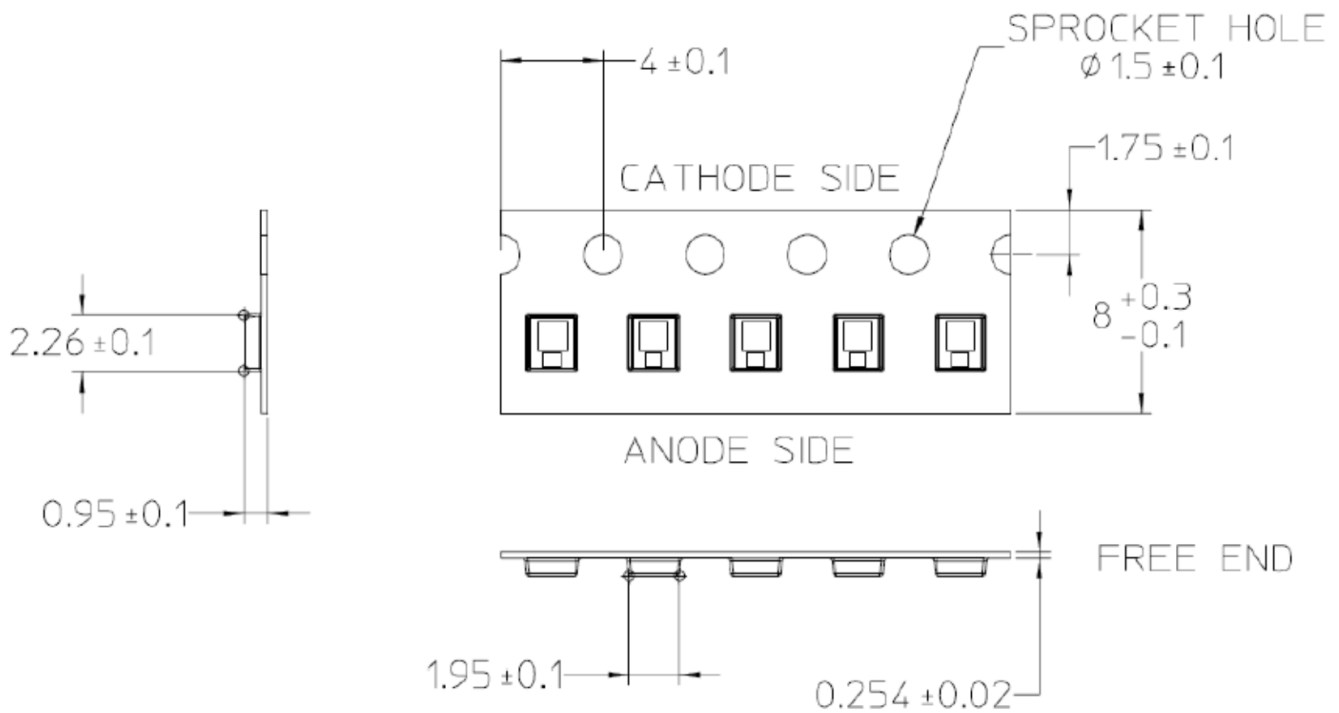
Figure 16. Tape dimensions.
