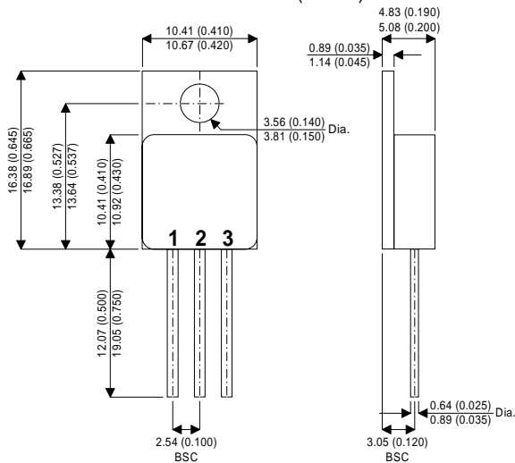
TO-257 Package Outline. Dimensions in mm (inches)
