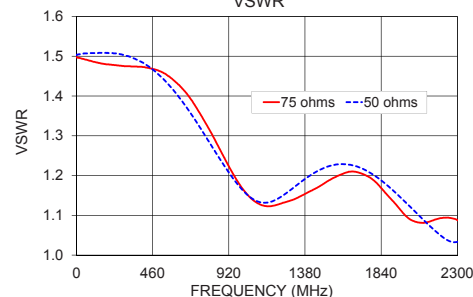
Z7550-FFNM+ VSWR
