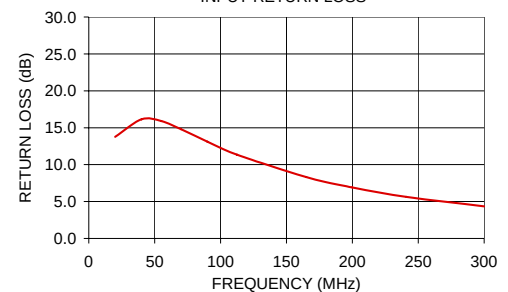
TC16-1T+ INPUT RETURN LOSS
