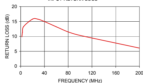
TC9-1+ INPUT RETURN LOSS
