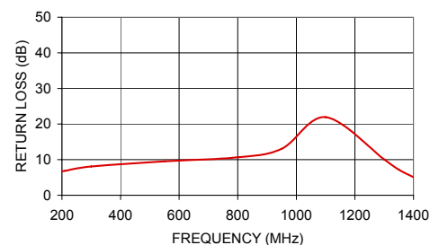
TC4-14+ INPUT RETURN LOSS
