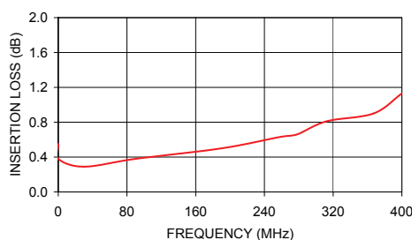
ADT3-6T INSERTION LOSS
