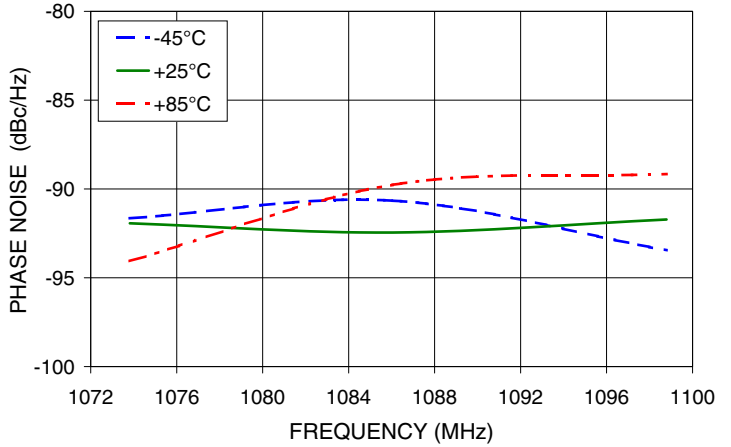
PHASE NOISE @ 1kHz offset (RF)
