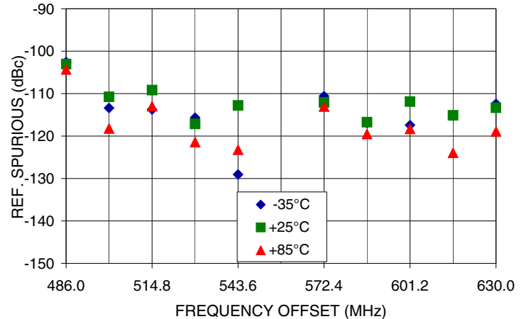
REFERENCE SPURIOUS Vs FREQ. OFFSET @ Fcar = 558MHz
