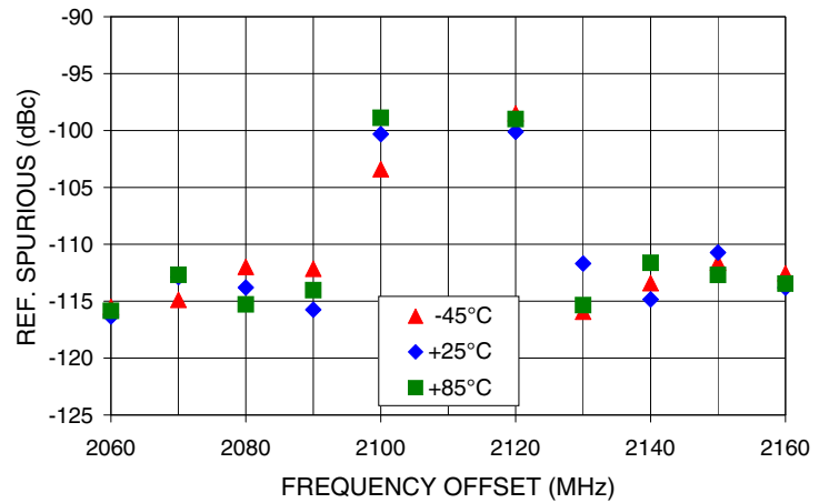
REFERENCE SPURIOUS Vs FREQ. OFFSET @ Fcar = 2110MHz
