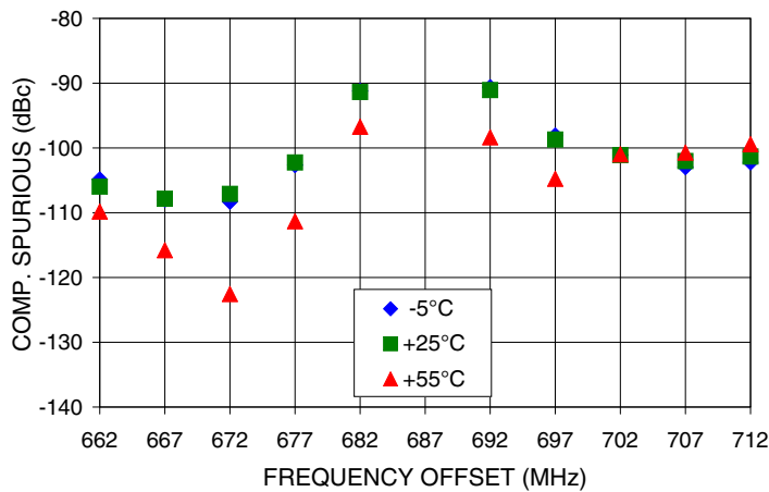
COMPARISON SPURIOUS Vs FREQ. OFFSET @ Fcar = 687MHz
