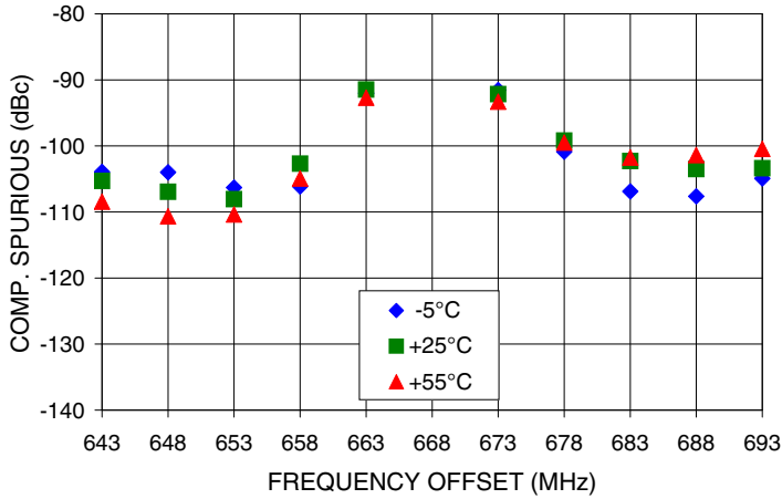
COMPARISON SPURIOUS Vs FREQ. OFFSET @ Fcar = 668MHz
