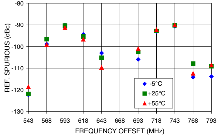
REFERENCE SPURIOUS Vs FREQ. OFFSET @ Fcar = 668MHz
