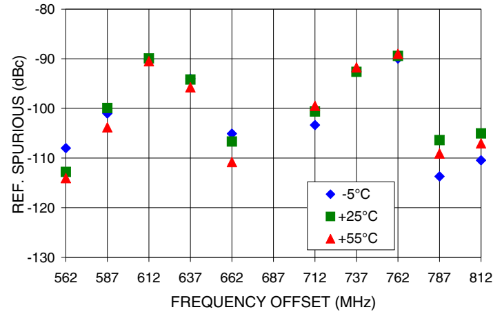
REFERENCE SPURIOUS Vs FREQ. OFFSET @ Fcar = 687MHz
