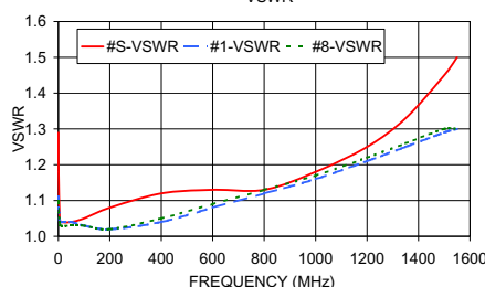
ZCSC-8-152+ VSWR
