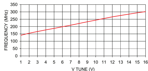
ZOS-300 FREQUENCY vs. TUNING VOLTAGE
