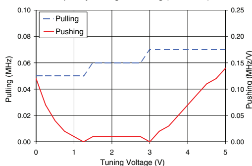
ROS-1000C-519+ Frequency Pulling & Pushing (Vcc ± 5%)
