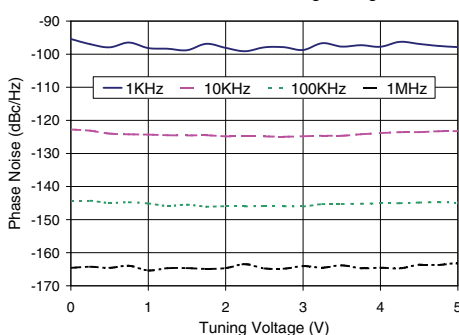
ROS-1000C-519+ Phase Noise Vs. Tuning Voltage
