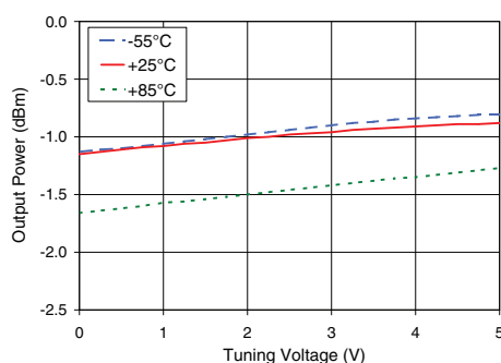
ROS-1000C-519+ Power Output
