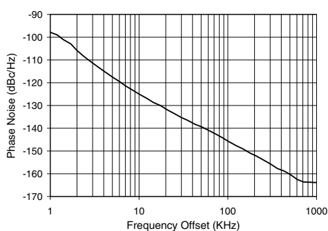
ROS-1000C-519+ Phase Noise
