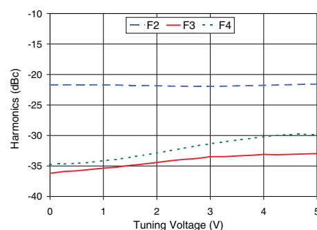
ROS-1000C-519+ Harmonics Level
