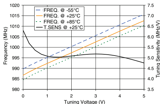
ROS-1000C-519+ Frequency and Tuning Sensitivity
