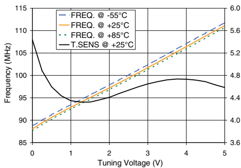
ROS-102-919+ Frequency and Tuning Sensitivity
