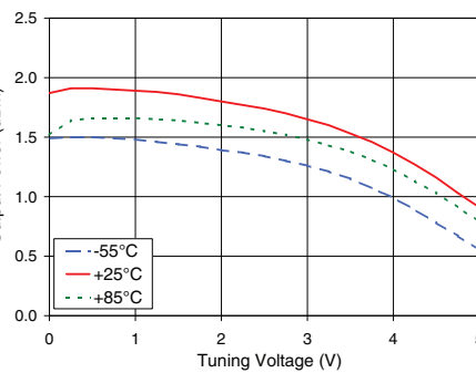
ROS-102-919+ Power Output
