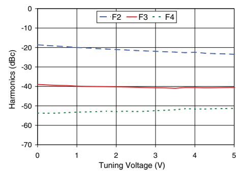
ROS-102-919+ Harmonics Level
