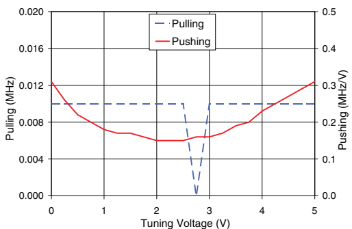
ROS-102-919+ Frequency Pulling & Pushing (Vcc ± 5%)
