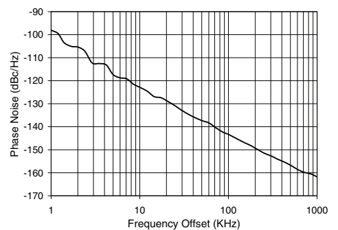
ROS-102-919+ Phase Noise
