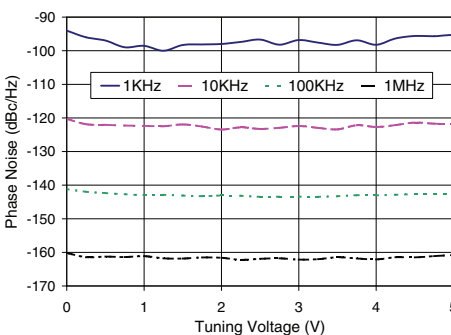
ROS-102-919+ Phase Noise Vs. Tuning Voltage
