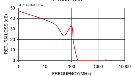
SALF-116 RETURN LOSS
